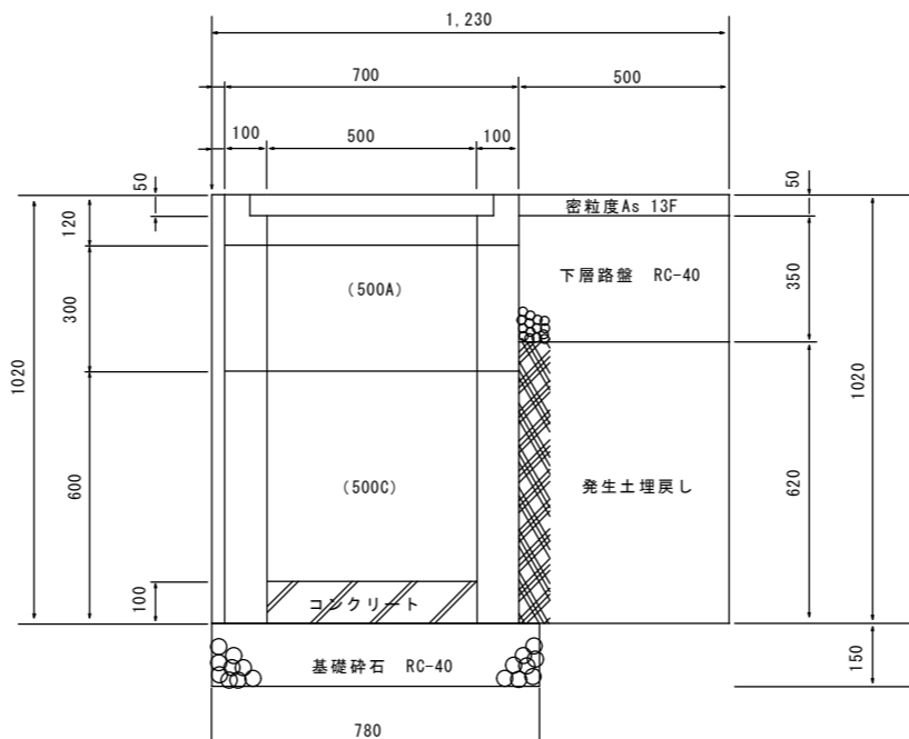
集水柵 500A+C (G縁塊) (1:10)
